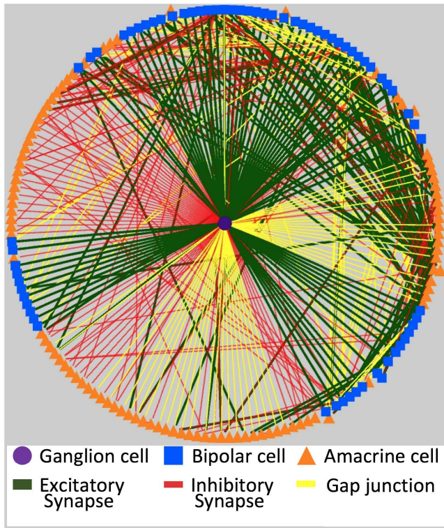
Fig. 3. Connectivity diagram of the neural network model, showing the ON ganglion cell considered in this study and every presynaptic cell (with the morphology depicted in Fig. 2), as extracted from the connectomics dataset. The node at the center is the ON ganglion cell and the nodes on the outside of the circular diagram are bipolar cells (blue) and amacrine cells (orange). The edges represent connections, including ribbon synapses (green), conventional synapses (red), and gap junctions (yellow).
