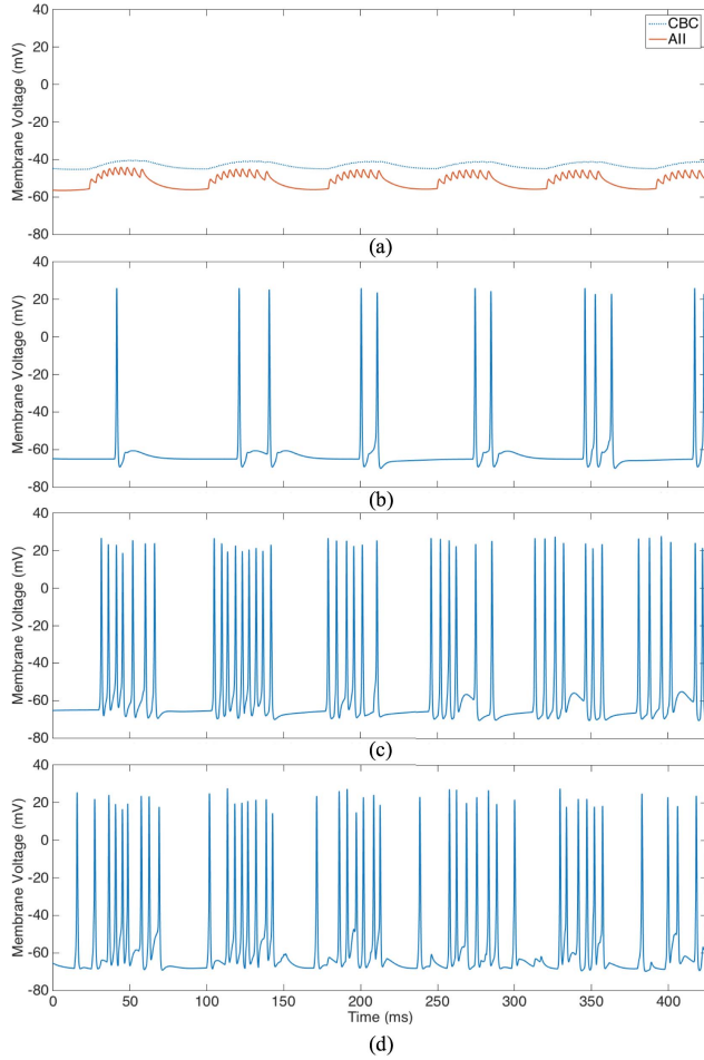
Fig. 7. Induced spontaneous activity in the retina neural network model without electrical stimulation intervention, showing the membrane potential for (a) a single cone bipolar cell coupled to an All cell (reproduction of results in [37] with gap junction conductance of 500 pS); (b) ganglion cell that is post-synaptic to the bipolar cell in (a), showing induced spontaneous firing; (c) the same ganglion cell as plotted in (b), but with all 47 All amacrine cells integrated into the model, coupled with CBCs appropriately via gap junctions, and all excitatory synapses included in the neural network model showing increased firing; and (d) the same as in (c) but with all excitatory and inhibitory synapses and gap junctions included in the neural network model, showing additional spontaneous activity.
