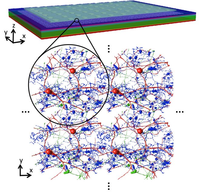
Fig. 2. Diagram of the multi-scale model of electrical stimulation of retinal tissue, including (Top) a discretized Admittance Method model consisting of a layered structure describing the retina and a 6 \times 10 electrode array placed 0.05 \text{ mm} away from the retina surface, and (bottom) a rendering of the NEURON model of an ON ganglion cell network, which was tiled to populate the entire ganglion cell, inner plexiform, and bipolar cell layers beneath the electrode array. This resulted in 888 cellular networks, each simulated independently.
